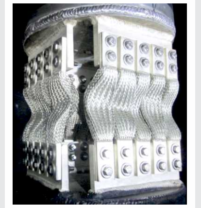
Braided Flexible Connection
