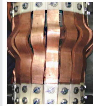
Laminated Flexible Connection
