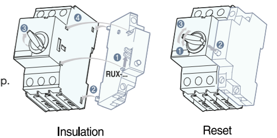
Insulation barrier
