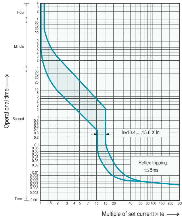
TCMS-32AF Tripping Curve
