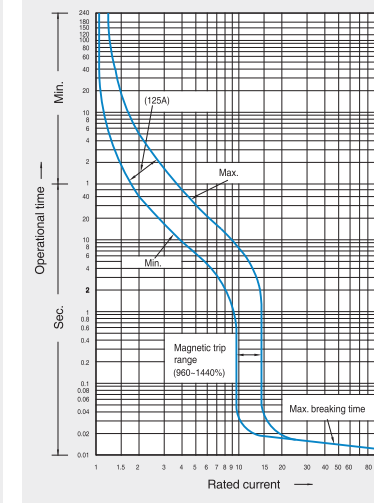
Rated current: 125A
