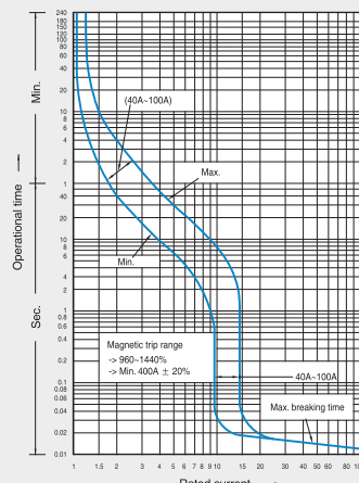
Rated current: 40-100A
