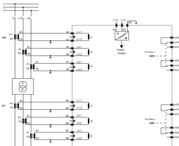
Fig. 3.1: Connection Diagram.
