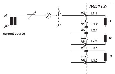
Fig. 6.2: Inrush blocking
