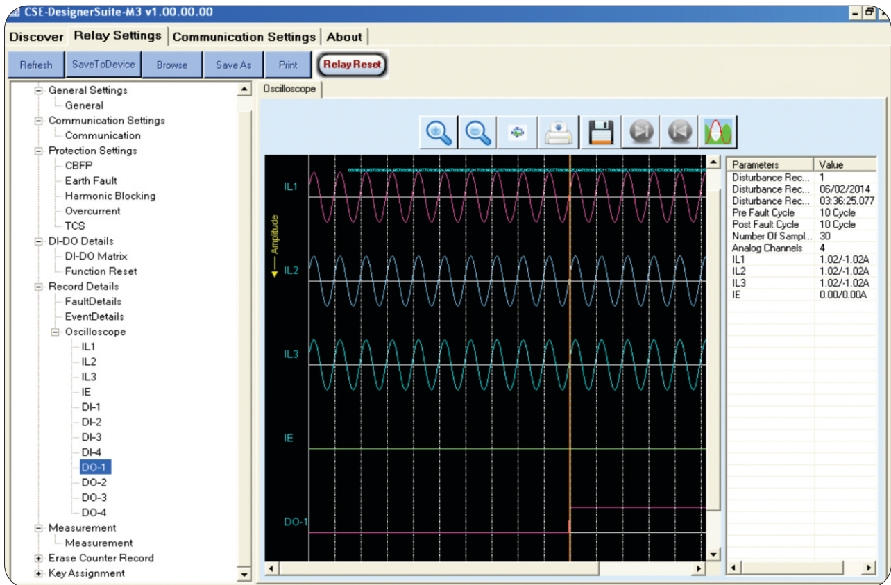
(Figure 5) (Disturbance Recording on PC software)
